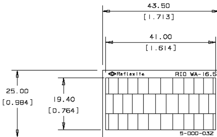
Lens Array Schematic
