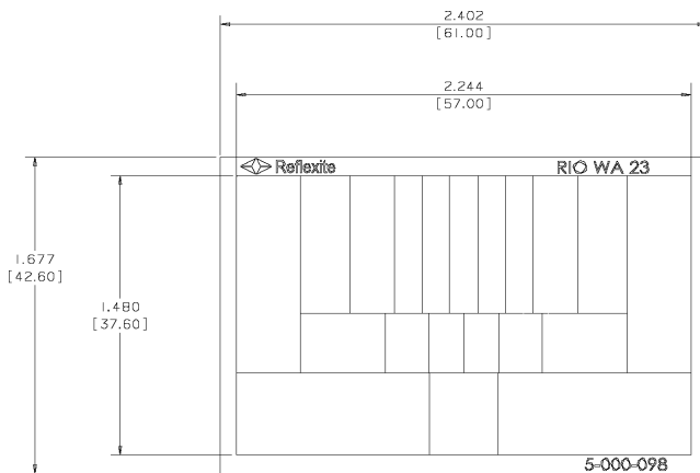
Lens Array Schematic
