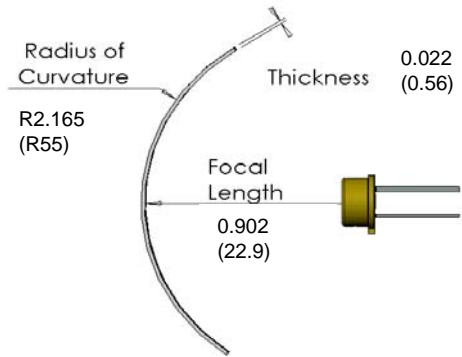
Recommended Installation
